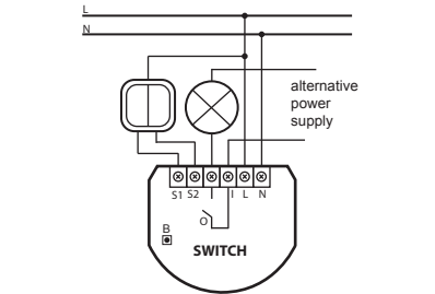
Fig.1 Wiring diagrams for Fibaro Switch.
