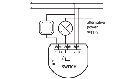
single switch - option with an alternative power supply for the load
