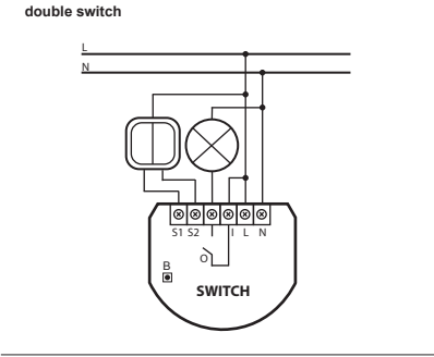
double switch - option with an alternative power supply for the load
