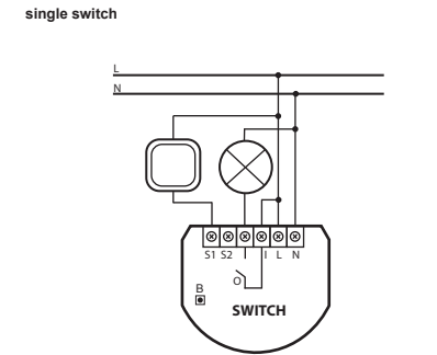
single switch - option with an alternative power supply for the load
